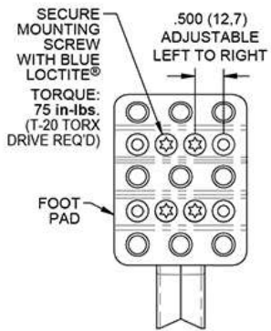
FOOT PAD DETAIL
